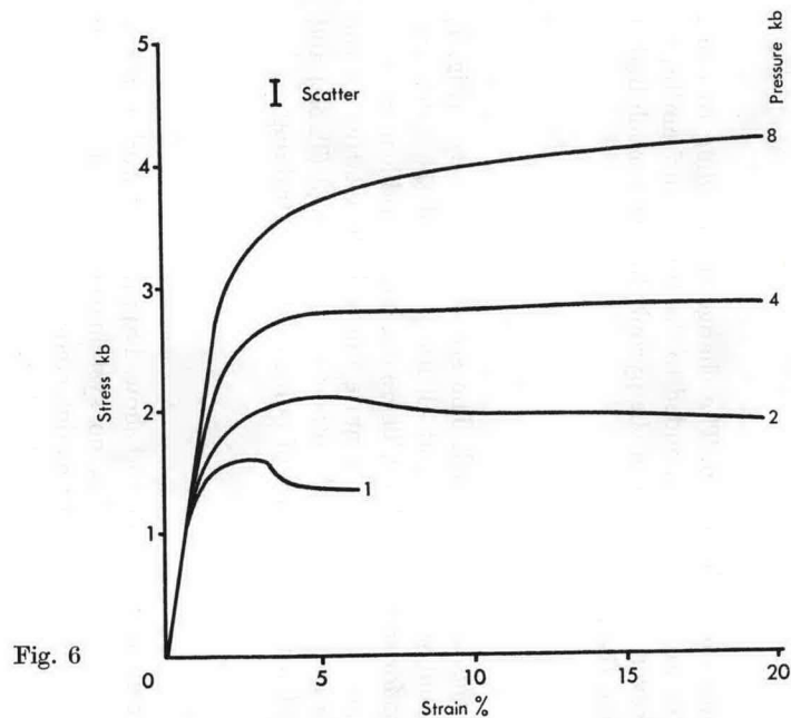
Fig. 6. Stress-strain curves for pyrophyllite at room temperature and confining pressures shown
